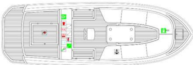
MAIN DECK PLAN SCALE 1:25
