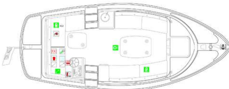
MAIN DECK PLAN SCALE 1:25
