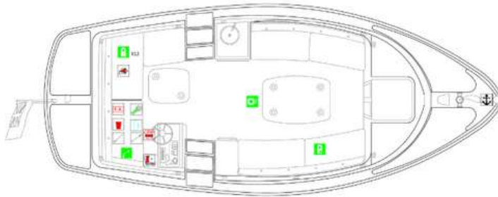
MAIN DECK PLAN SCALE 1:25
